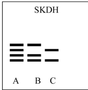
Scheme 1. — Presentation of SKDH zymogram pattern of bean genotypes
