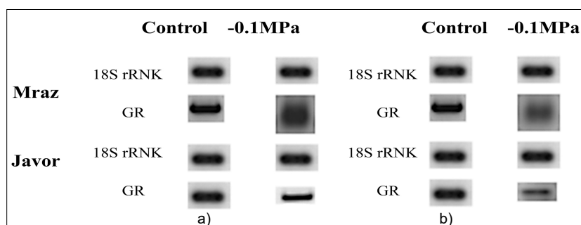
Fig 6: The influence of osmotic stress on the expression of the GR gene in the shoots (a) and roots (b) of field pea varieties.
