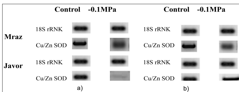
Fig 4: The influence of osmotic stress on the expression of the Cu/Zn SOD gene in the shoots (a) and roots (b) of field pea varieties.
