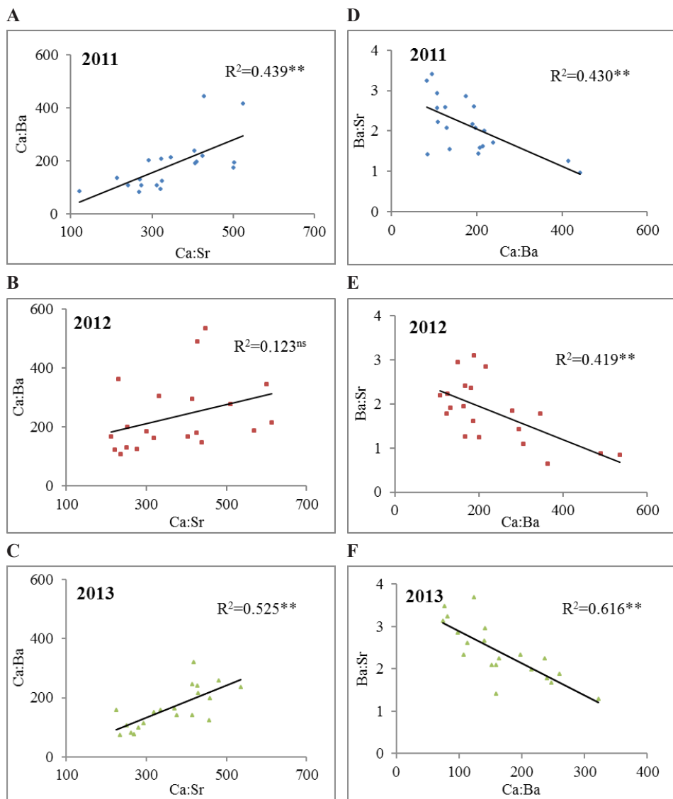
Figure 1. Pearson's liner correlation coefficients among ratios of concentrations of Ca:Ba and Ca:Sr (A, B, C), and Ba:Sr and Ca:Ba (D, E, F) in the whole grain of Aegilops and Triticum species in three experimental years. Ratios between Ba:Sr and Ca:Sr were not statistically significant and therefore are not shown.
